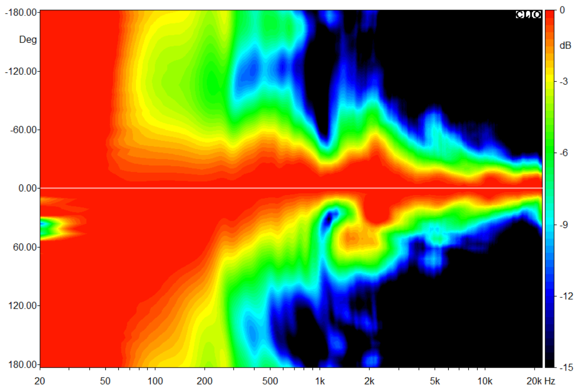
Directivity M8-C Vertical position Vertical directivity
