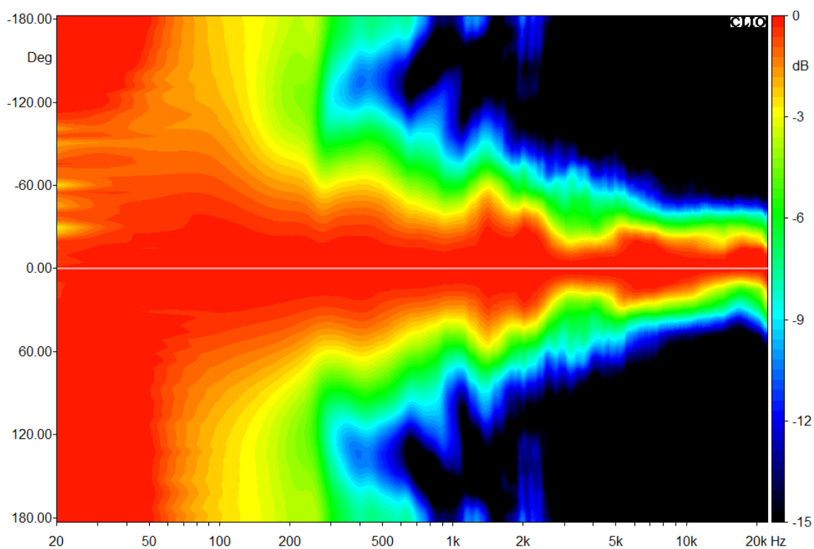
Directivity M8-C Vertical position Horizontal directivity
