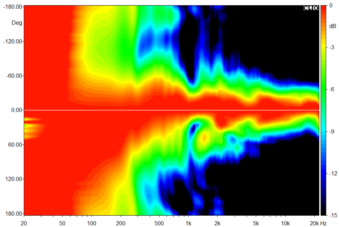
Directivity M8-C Horizontal position Horizontal directivity
