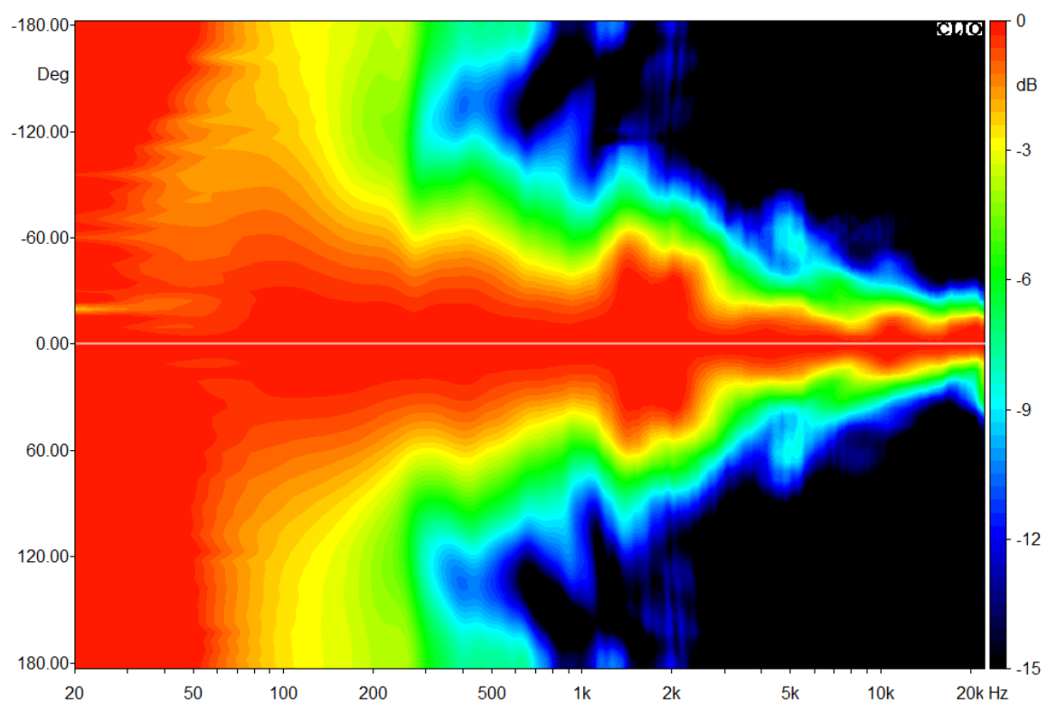
Directivity M8-C Horizontal position Vertical directivity
